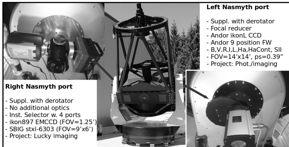
Figure 1: The 1.4m telescope (middle) and the two ports with image-derotator.
